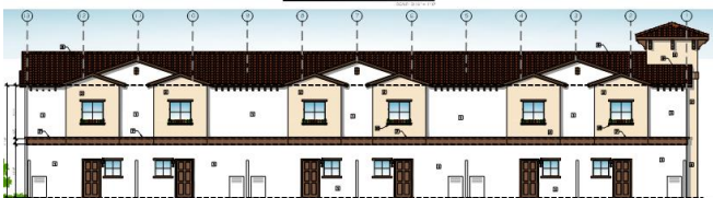
REAR ELEVATION (BUILDING C)
