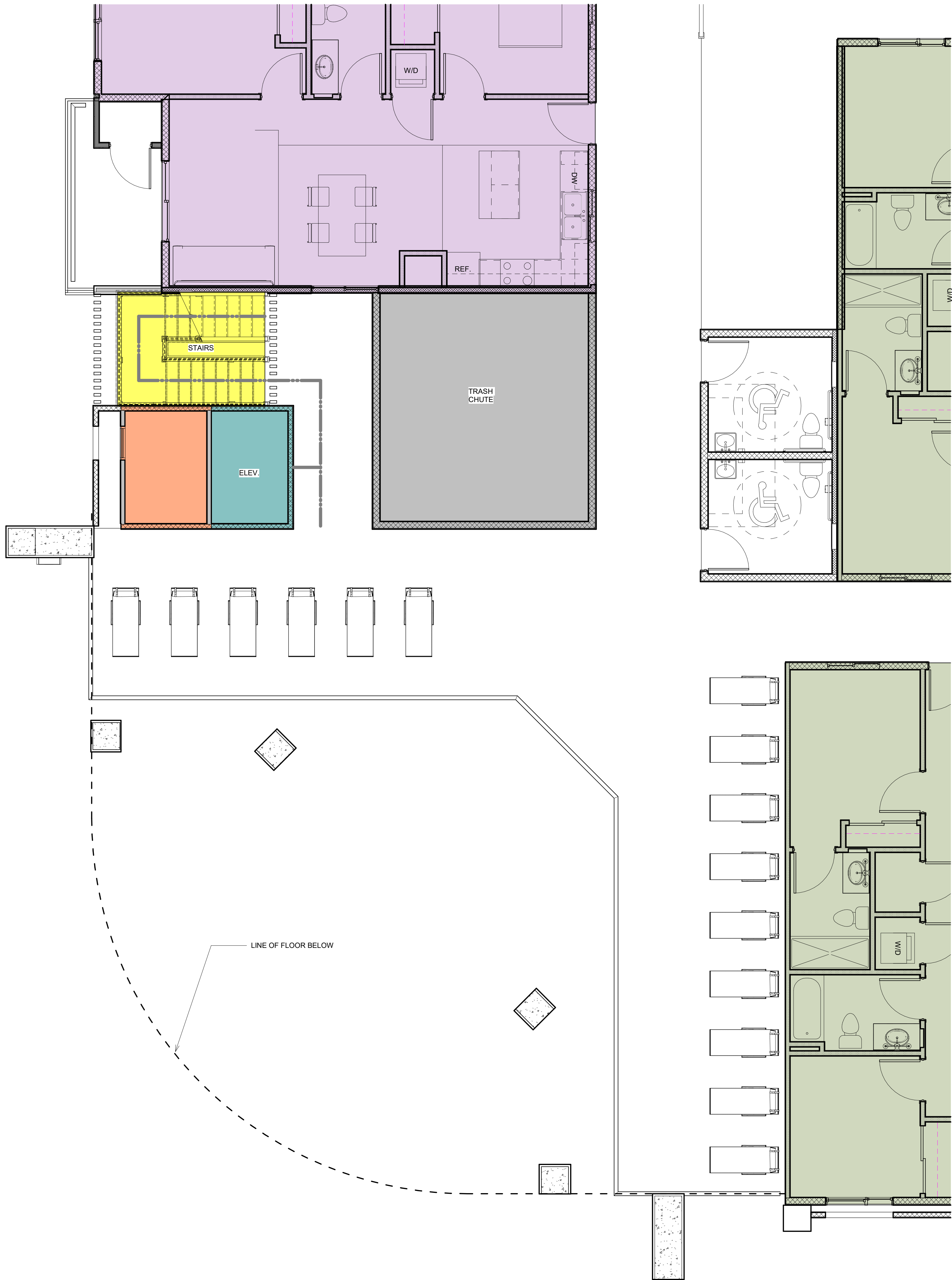
Second Floor Patio Plan 1/4" = 1'-0"
