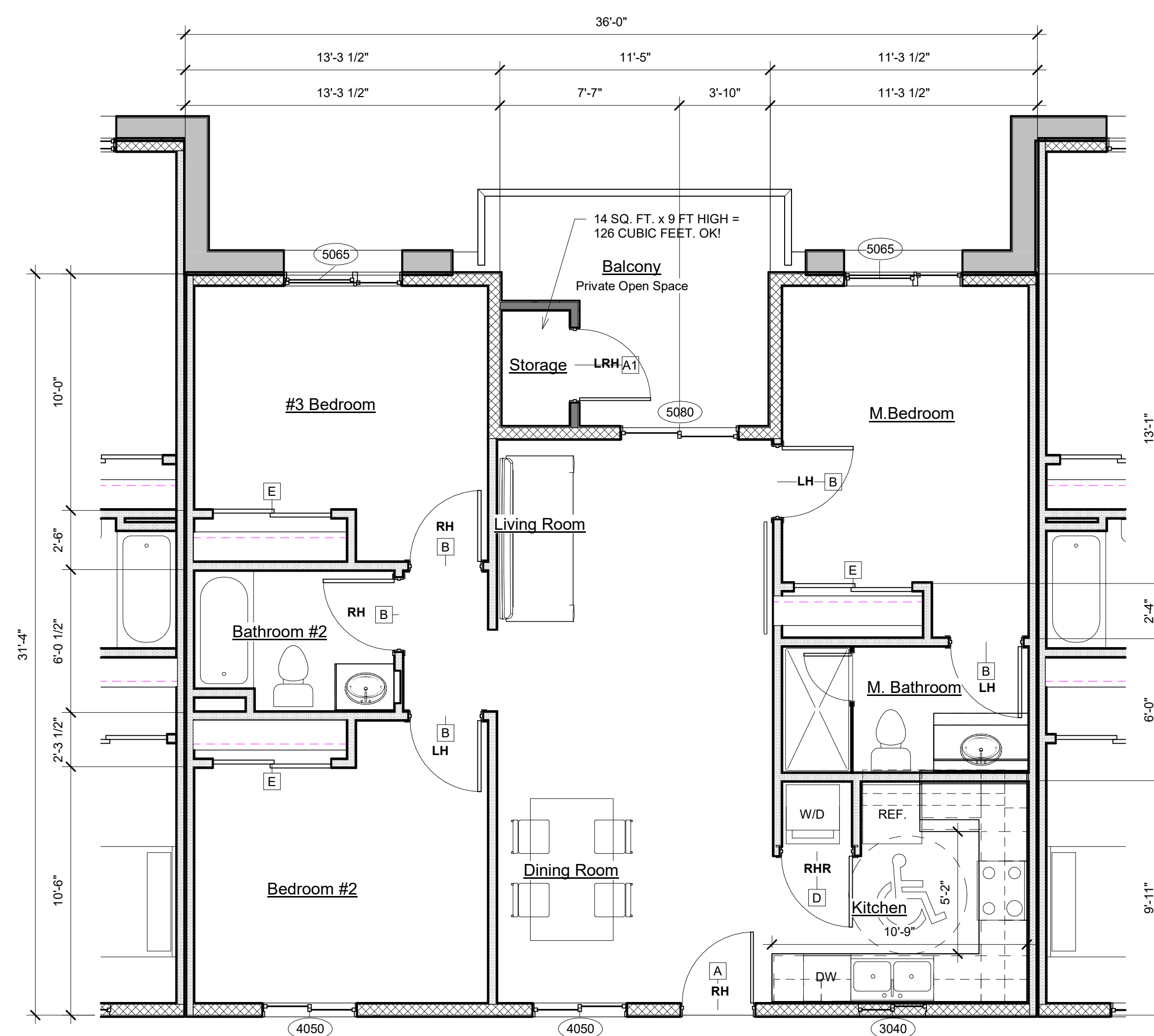
Typical 3-Bedroom Floor Plan - Option "B" 1/4" = 1'-0"
